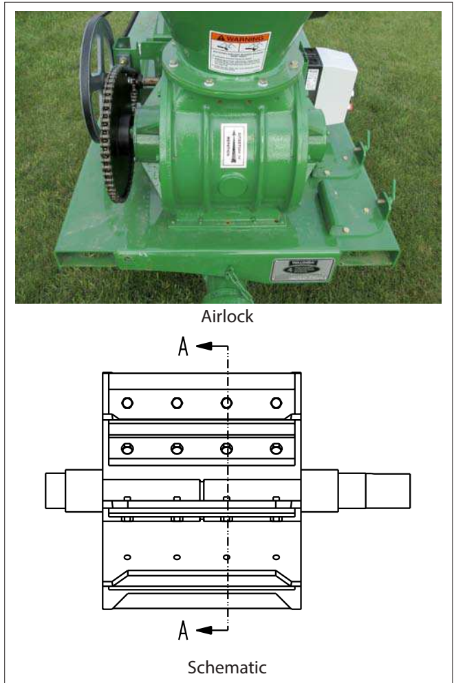
FIG. 34 TIP ADJUSTMENT
