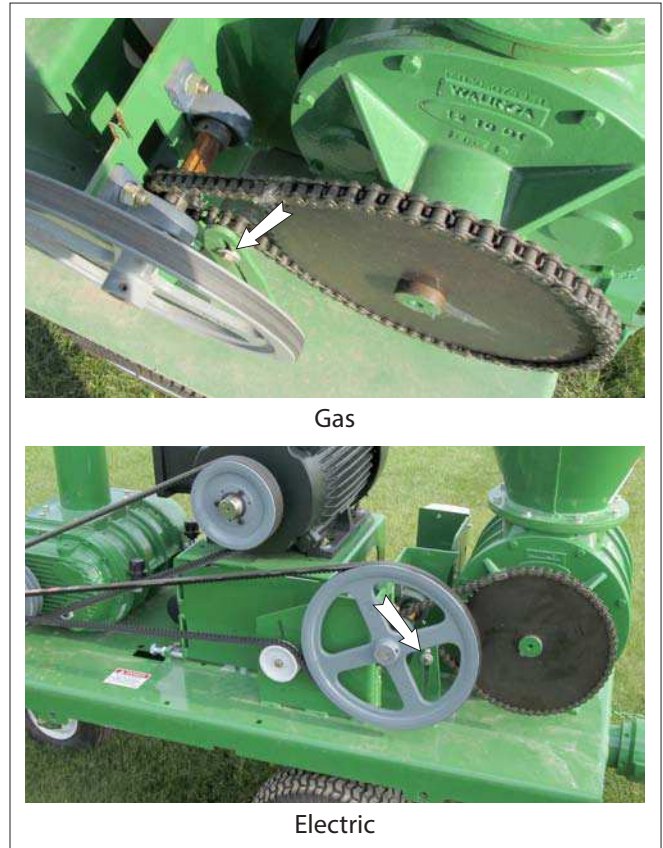
FIG. 30 CHAIN TENSION
